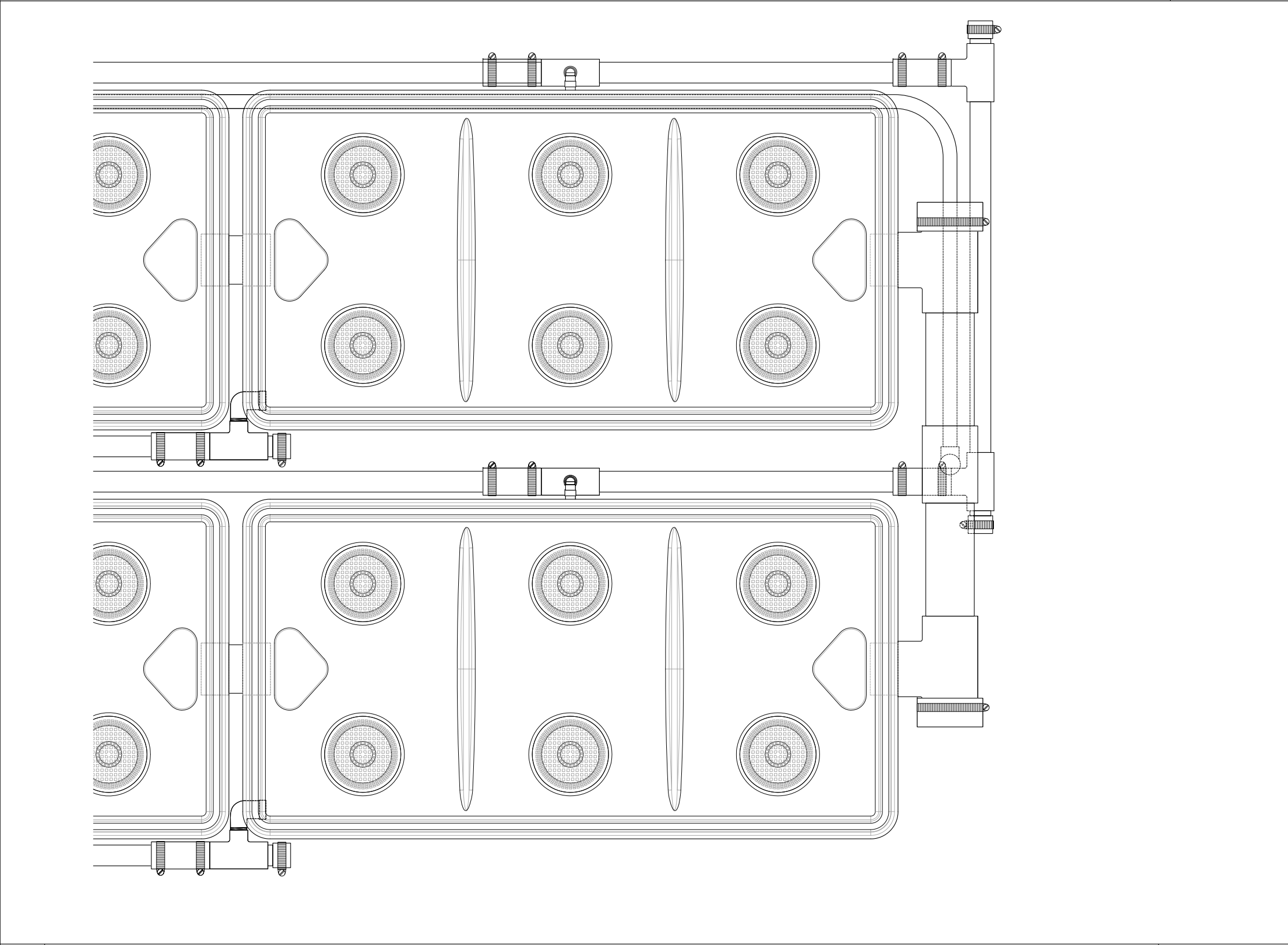
C ENLARGED VIEW SCALE: 1"-1/2"=1'-0"
