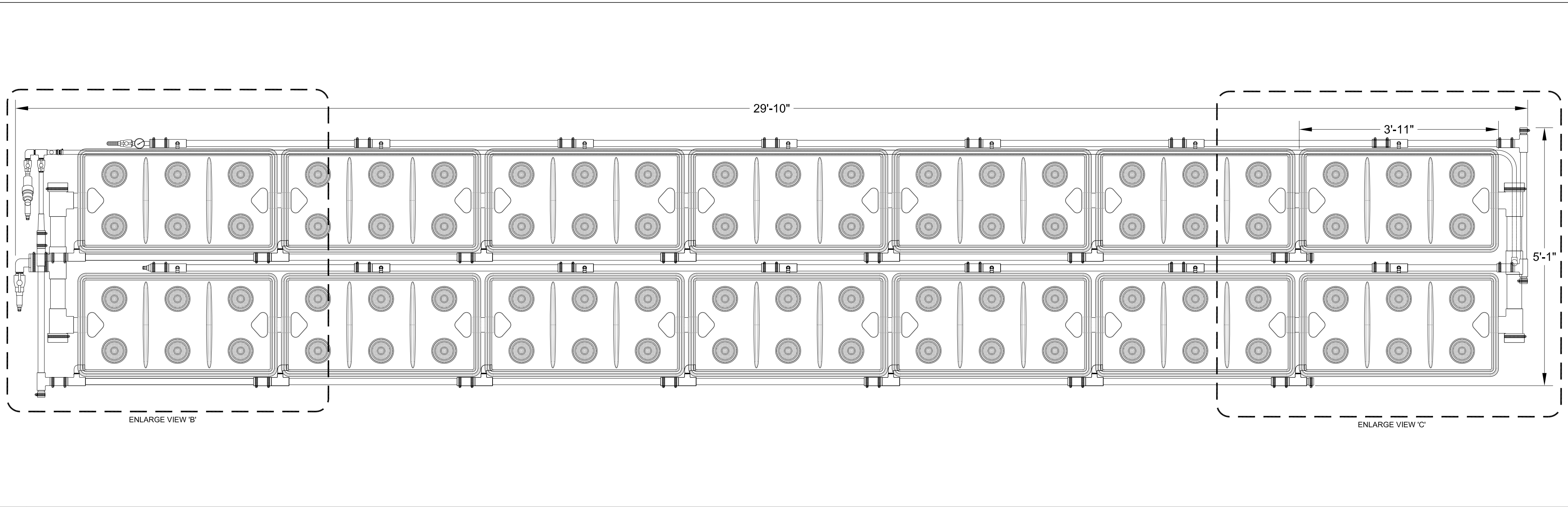
A OVERALL VIEW SCALE: 3/4"=1'-0"
